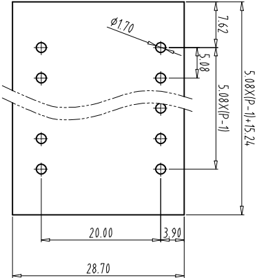
PCB Layout
